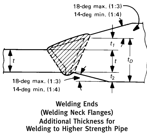
Fig. 14 Bevel for Combined Thickness
